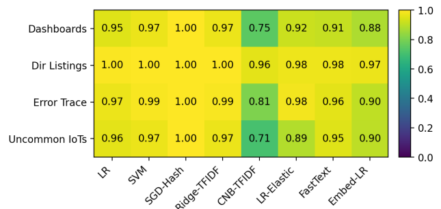
Figure 7: Pairwise prediction agreement between the best-performing model and all other classifiers, per dataset.
